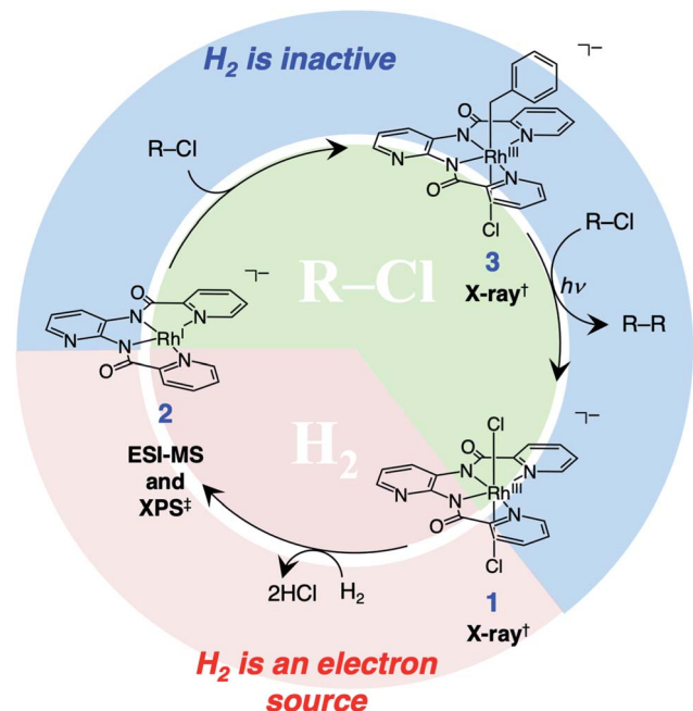
Fig. 4 A proposed mechanism of the photoinduced reductive homo-coupling of benzyl or allyl halides with H_2 catalysed by the ESC. †The structures of 1 and 3 were determined by X-ray analysis. ‡2 was characterised by ESI-MS and XPS.
