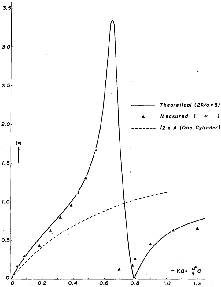
Fig. 7 The amplitude ratio (wave amplitude/heaving amplitude)
