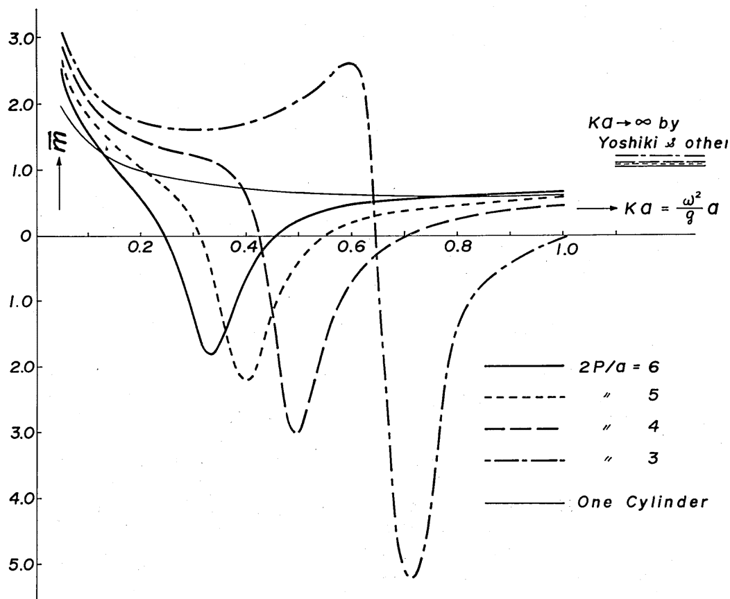
Fig. 8 Added mass coefficient
