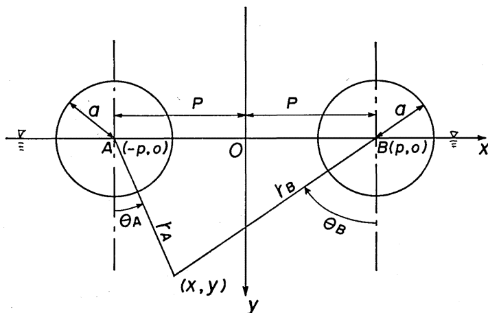
Fig. 1 Coordinate system.
