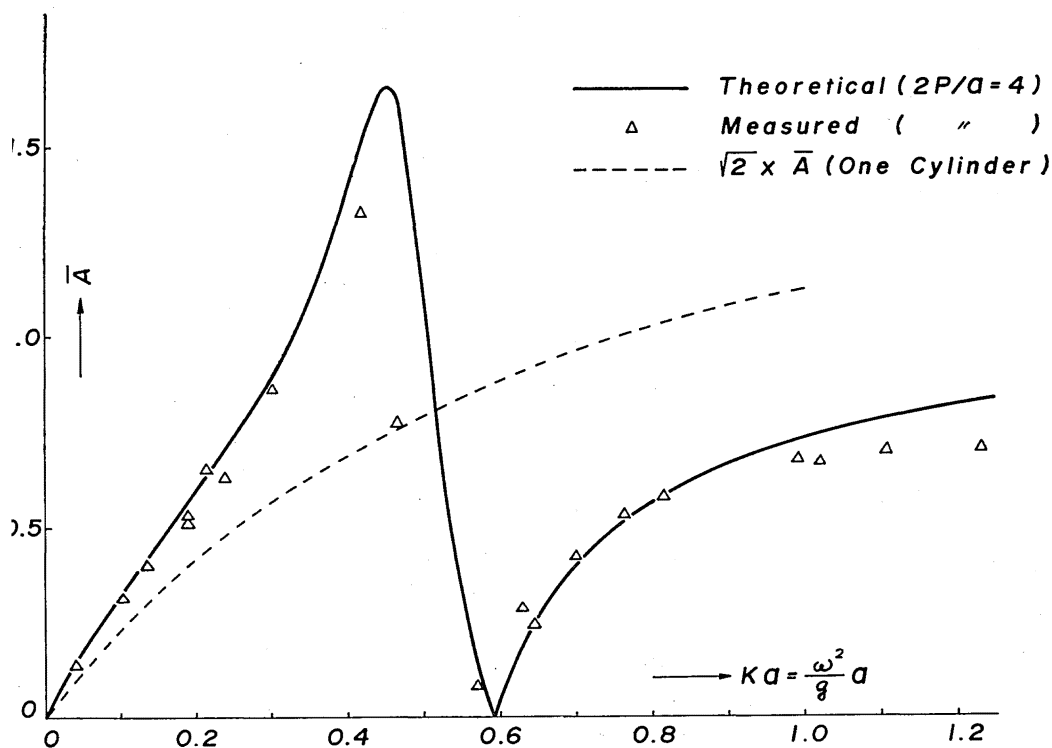
Fig. 6 The amplitude ratio (wave amplitude/heaving amplitude)
