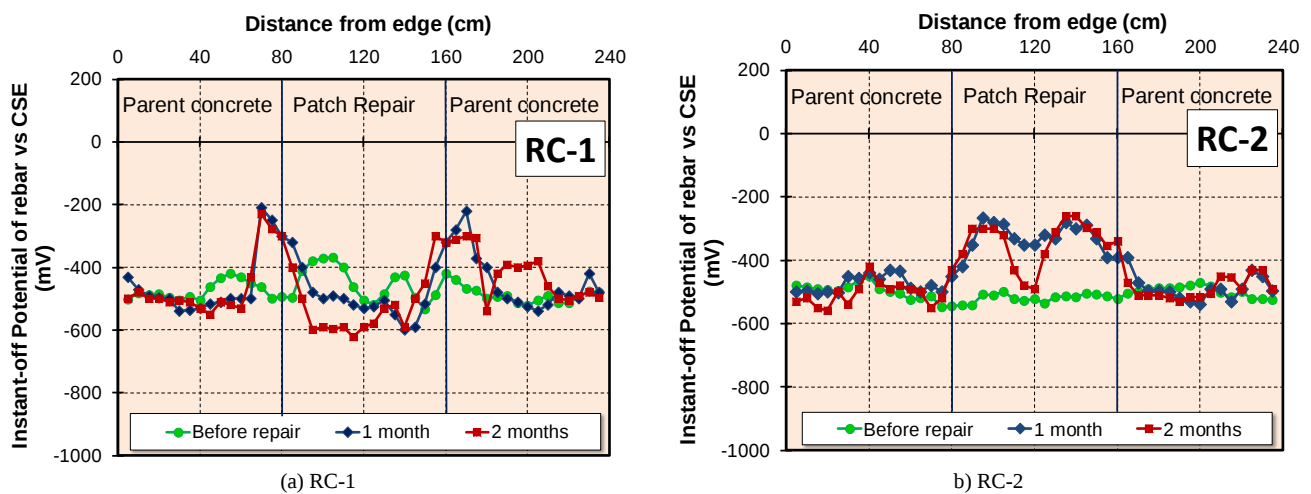
Figure 8. Instant-off potential of the rebar (The sacrificial anodes were in the patch repair, Stage I)
