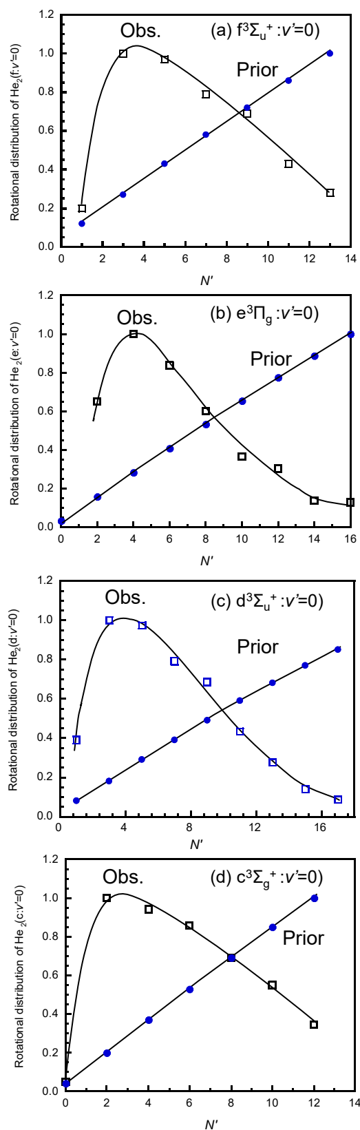
Fig. 7. Observed and statistical prior rotational distributions of the \text{He}_2(\text{f}: v'=0) , \text{He}_2(\text{e}: v'=0) , \text{He}_2(\text{d}: v'=0) , and \text{He}_2(\text{c}: v'=0) states in the \text{He}_2^+/2\text{e}^- CRR reaction
