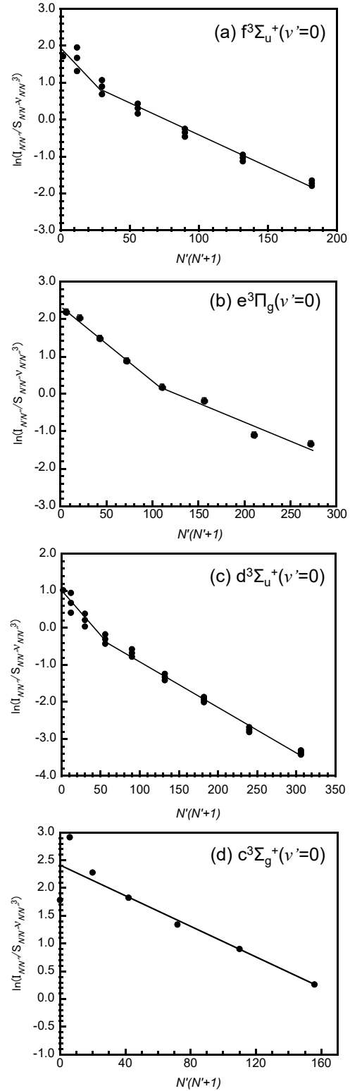
Fig. 6. Estimation of effective rotational temperatures from the slopes of \ln(I_{N'N''}/\nu_{N'N''}^3 S_{N'N''}) against N'(N' + 1) for the \text{He}_2(\text{f}; v'=0) , \text{He}_2(\text{e}; v'=0) , \text{He}_2(\text{d}; v'=0) , and \text{He}_2(\text{c}; v'=0) states in the \text{He}_2^+/2\text{e}^- CRR reaction.
