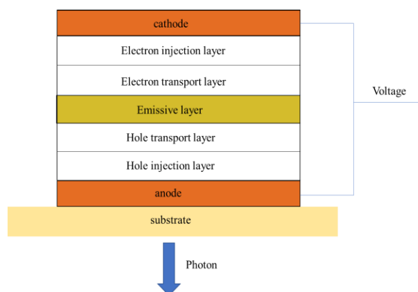
Figure 3. OLEDs design
