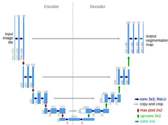
Figure 3. U-Net Architecture.
