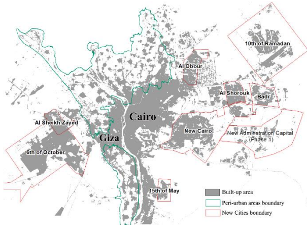
Figure 2. Greater Cairo and its urban extent in 2021
