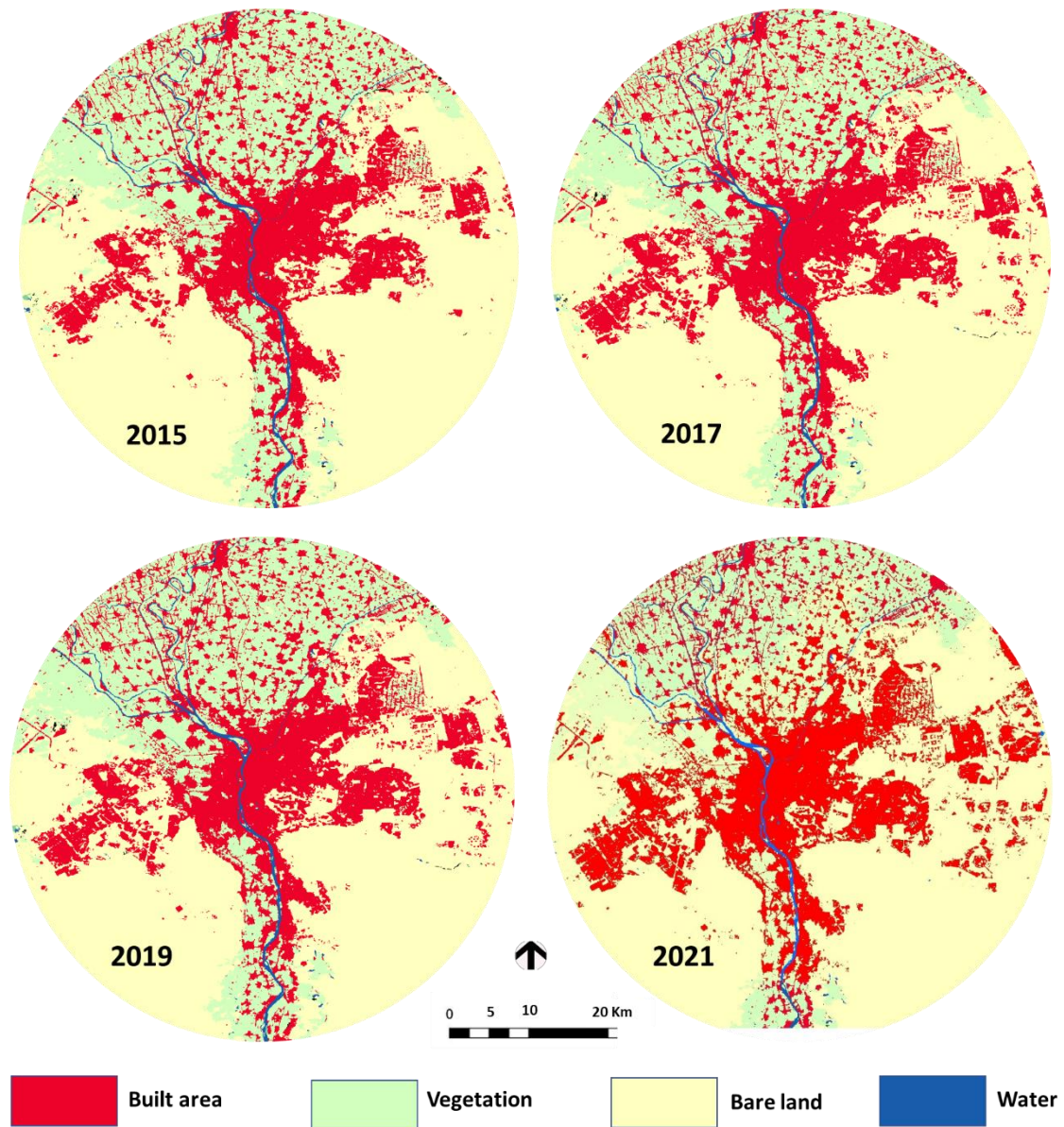
Figure 4. The change in land cover between 2015-2021.
