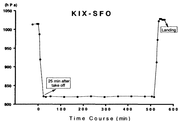
Fig.5. The changes in the cabin pressure during a flight (flight No.: UA810) from Kansai International Airport to San Francisco International Airport on February 25, 1998.
