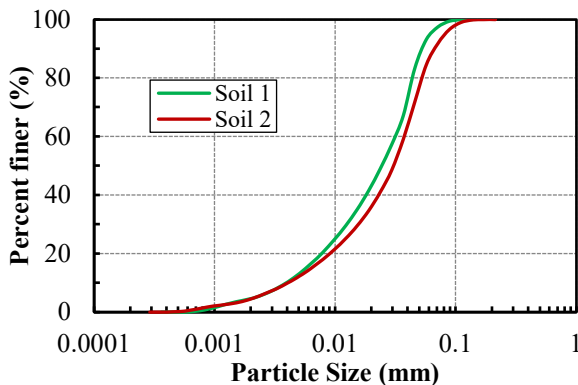
Figure 3. Grain size distribution.
