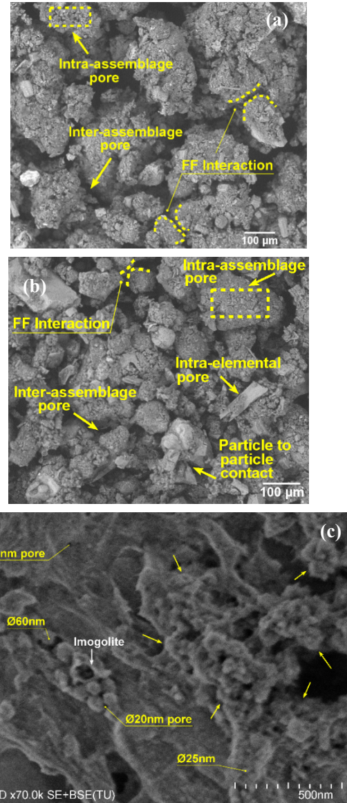
Figure 5. (a) SEM image of Soil 1 showing inter and intra assemblage pores and face to face (FF) contact. (b) SEM image of Soil 2 showing different types pores, face to face (FF) and particle to particle interaction. (c) FE-SEM image of Soil 2 showing presence of 25nm and 60nm allophane domains, imogolite fibres and presence of mesopores. Arrows indicate aggregation of allophane domains.
