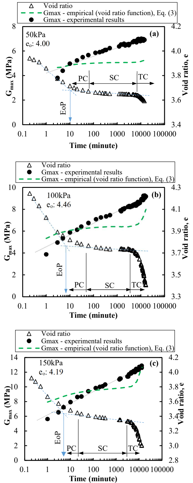
Figure 6. Variation of G_{\max} with time (a) Soil 1 – 50 kPa. (b) Soil 1 – 100 kPa. (c) Soil 1 – 150 kPa.
