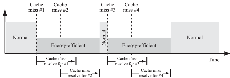
図 7 E-DFUG と DFUG の違い Fig. 7 The difference between E-DFUG and DFUG
