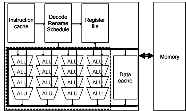
Figure 2. Instruction collapsing
