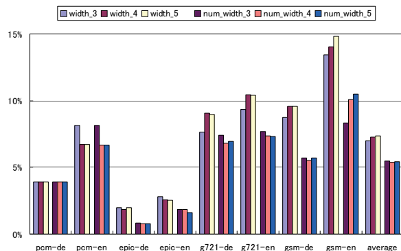
Figure 10. IPC speedup
