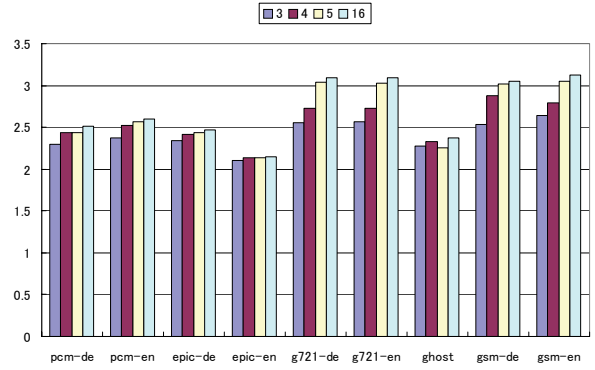
Figure 4. The number of instruction per strand
