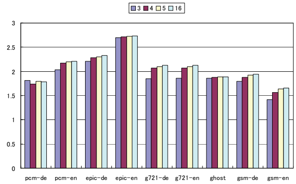
Figure 5. The number of operands per strand
