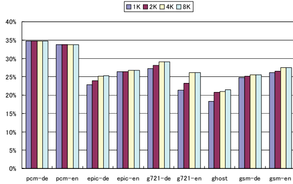
Figure 7. Strand cache hit rate
