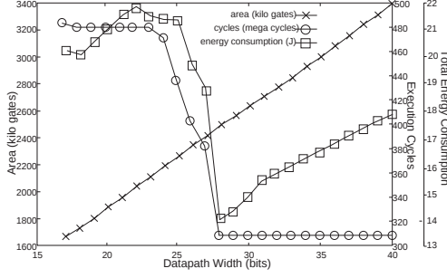
Fig. 7 Energy consumption, execution cycles and area (gates) for MPEG2 decoder
