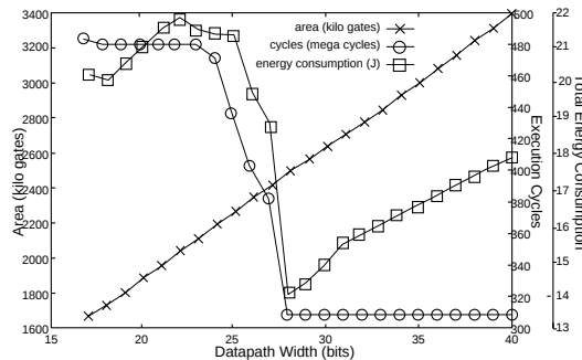
Figure 7: Energy consumption, execution cycles and area (gates) for MPEG-2 decoder
