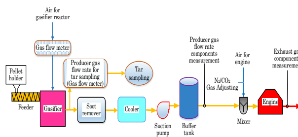
Fig. 2: The downdraft gasifier system block diagram
