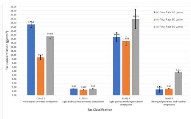
Fig. 7: Classification of tar according to molecular weight, with a moisture content of 2 wt.% at air flow rates of 40, 60, and 80 Liters/min respectively
