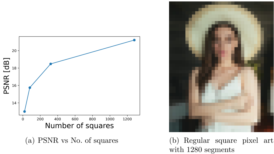
FIGURE 5. Quantitative and visual qualities of regular square pixel art: (a) Peak signal-to-noise ratio (PSNR) monotonically increases with the number of squares, and (b) the image with 1280 squares captures the outline of the original image in Figure 2(a)
