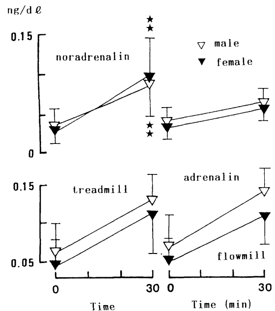
Fig. 5. Catecholamine during walking on treadmill and in flowmill.
