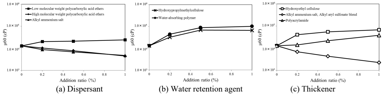
Figure 5. Relationship between viscosity and addition ratio of each surfactant
