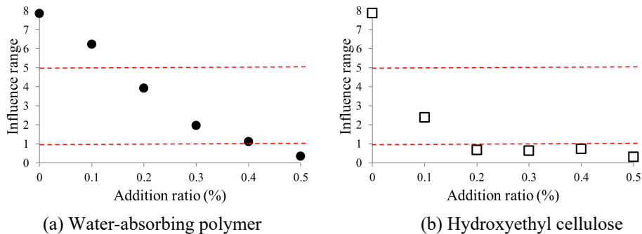
Figure 7. Modification effect by suction test: circular to cone-shape
