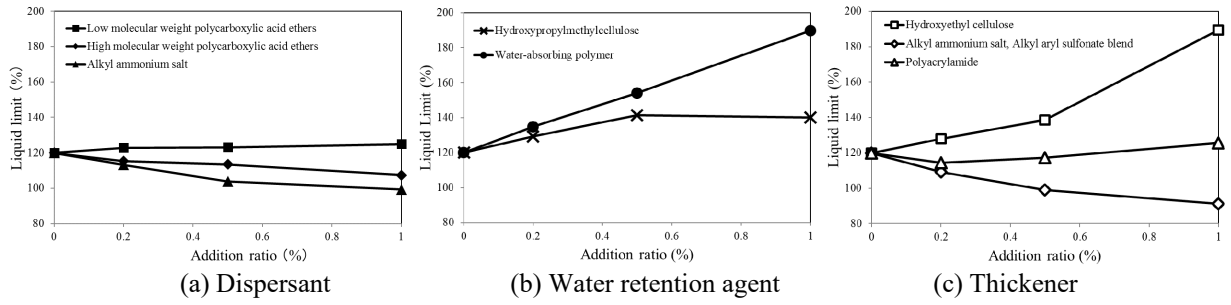
Figure 3. Relationship between liquid limit and addition ratio of each surfactant
