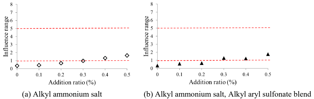
Figure 8. Modification effect by suction test: sharp to cone-shape
