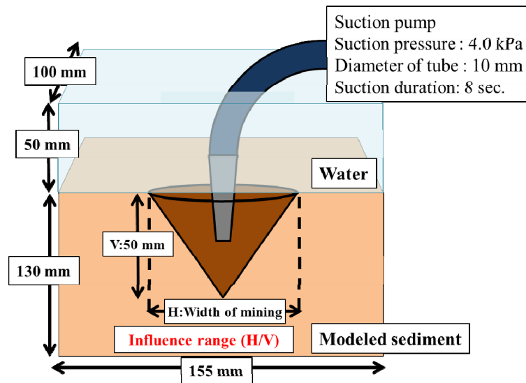
Figure 2. Conceptual diagram of suction pump test
