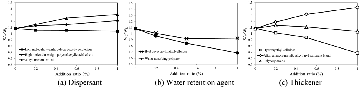
Figure 4. Relationship between the ratio of water content to liquid limit ( W_c/W_L ) and addition ratio of each surfactant
