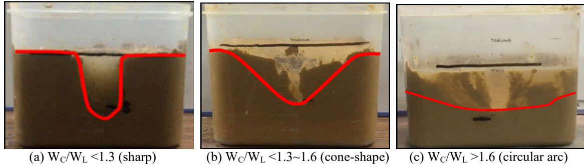
Figure 1. Classification of deformation behavior of simulated soil based on the water content ( W_c ) and the liquid limit ( W_L )
