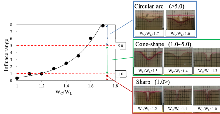
Figure 6. Definition of influence range for 3 types based on W_C/W_L : circular arc, cone-shape, and sharp
