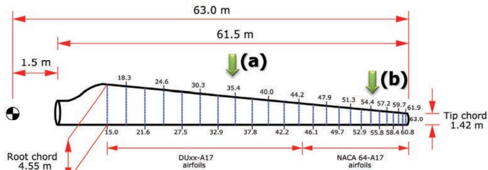
Radial distribution of blade elements for NREL-5 MW turbine
