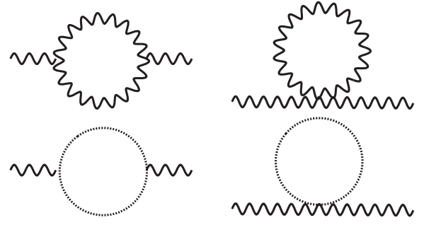
FIG. 4. Feynman diagrams for \Pi_{11}^{\text{Gauge}, cc} , \Pi_{33}^{\text{Gauge}, cc} , and \Pi_{3Q}^{\text{Gauge}, cc} . The wavy and dotted lines correspond to gauge fields and Faddeev-Popov ghost fields, respectively.
