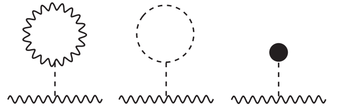
FIG. 1. Feynman diagrams for tadpole contributions to \Pi_{11}(0) and \Pi_{33}(0) and their counterterms.
