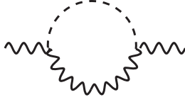
FIG. 3. Feynman diagrams for \Pi_{11}^{\phi V} , \Pi_{33}^{\phi V} , and \Pi_{3Q}^{\phi V} . The internal lines correspond to \phi and gauge fields.
