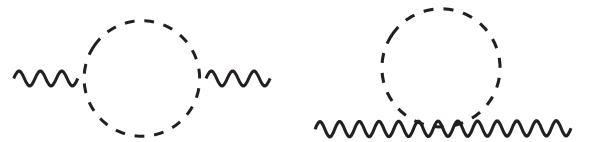
FIG. 2. Feynman diagrams for \Pi_{11}^{\varphi\varphi} , \Pi_{33}^{\varphi\varphi} , and \Pi_{3Q}^{\varphi\varphi} . The internal lines correspond to \varphi fields.
