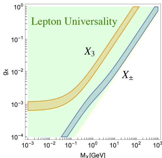
Figure 4. Regions excluded by the constraint of \mu/e lepton universality from the leptonic \tau decays at the 1\sigma and 2\sigma levels are shown in light yellow and light green, respectively. The regions favored by the muon g - 2 anomaly are also superimposed.
