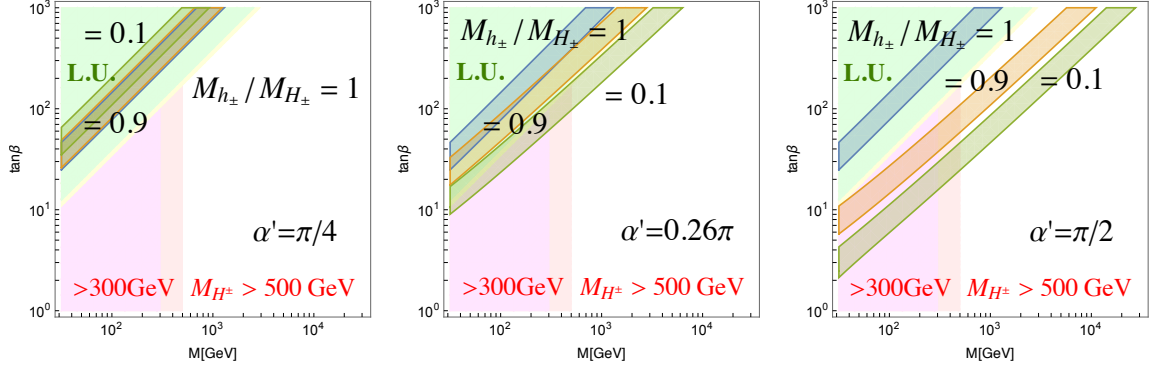
Figure 5. Parameter space favored by the muon g - 2 anomaly at 2\sigma level is plotted together with the constraint of the \mu/e lepton universality from the leptonic \tau decays at 1\sigma (light green) and 2\sigma (light yellow) levels (labeled by L.U.) as well as the LHC direct search in light magenta for M_{H^\pm} > 300 GeV and light pink for M_{H^\pm} > 500 GeV. We here take into account only the contribution of flavor-changing scalar bosons to \Delta a_\mu , and assume M^2 \equiv M_H^2 = M_A^2 = M_{H^\pm}^2 = M_{h^\pm}^2 for definiteness. The left, middle, right plots are for \alpha' = \pi/4, 0.26\pi, \pi/2 , respectively.
