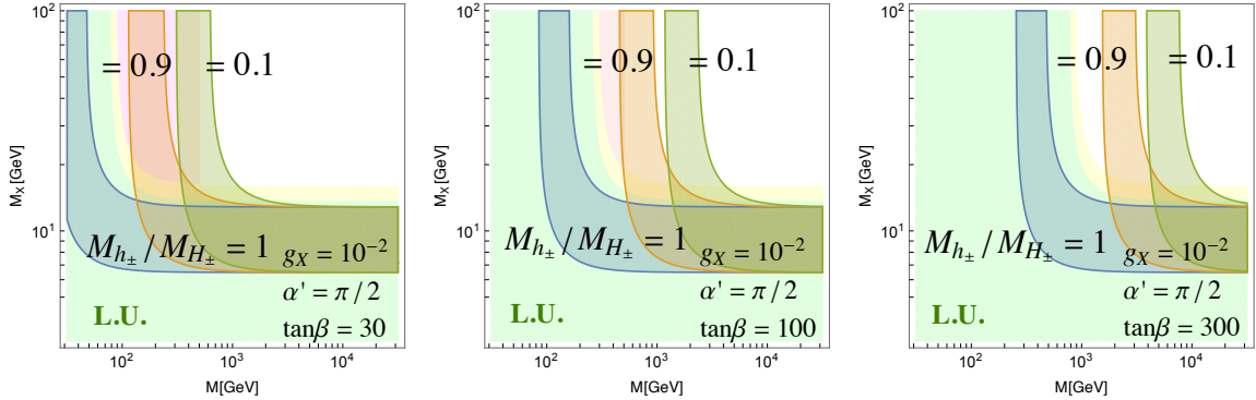
Figure 6. Parameter space favored by \Delta a_\mu for M_{h^\pm}/M_{H^\pm} = 1 (blue), 0.9 (orange) and 0.1 (green) and disfavored by the universality in leptonic \tau decays at 1\sigma (light green) and 2\sigma (light yellow) levels. The M_{H^\pm} > 500 GeV bound is drawn in light pink. These plots all assume g_X = 10^{-2} , \alpha' = \pi/2 and M^2 \equiv M_H^2 = M_A^2 = M_{H^\pm}^2 = M_{h^\pm}^2 for definiteness. The left, middle, right plots are for \tan \beta = 30, 100, 300 , respectively.
