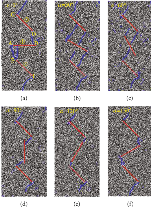
FIGURE 11: Initial crack propagation of the specimens containing three precracks.
