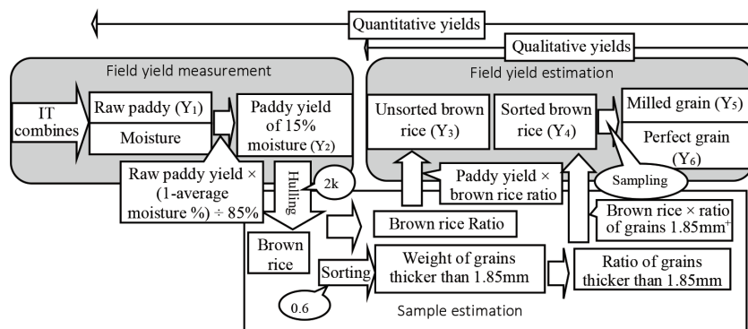
Fig. 2. Process of estimating the rice yields from raw paddy to milled and perfectly shaped grains. Source: Nanseki (2019a, p. 166)
