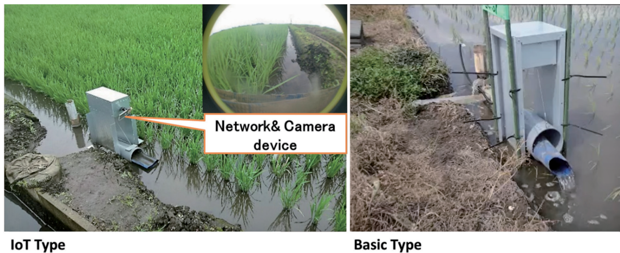
Fig. 6. Automatic Paddy Water Supply Systems.
