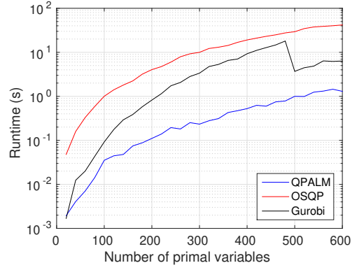
Fig. 1: Runtime comparison for random LPs of varying sizes.
