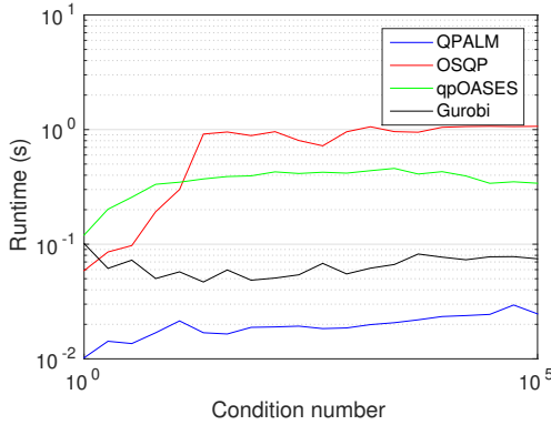
Fig. 3: Runtime comparison for random QPs with varying conditioning.
