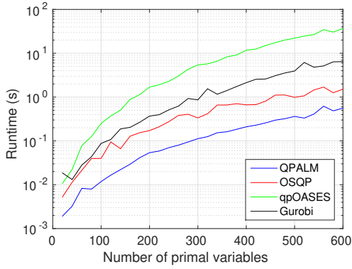
Fig. 2: Runtime comparison for random QPs of varying sizes.
