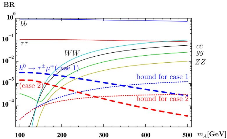
Fig. 1. The decay branching ratios of the lightest Higgs boson h^0 as a function of m_A at \tan\beta = 60 . The m_h is set to be 123 GeV. The dashed curves represent the branching ratio for h^0 \rightarrow \tau^\pm\mu^\mp in Case 1 and Case 2. The experimental upper constraint in Eq. (8) is plotted for each case as a dotted curve. The branching ratios for the other decay modes are also shown for Case 1.
