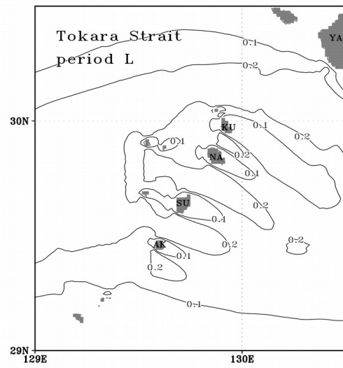
Fig. 2-9 Average ocean current power density (unit: kW/m 2 ) at 50 m depth during periods N and L (ECS East China Sea, AS Cape Ashizuri, SH Cape Shionomisaki, YA Yakushima, KU Kuchinoshima, NA Nakanoshima, SU Suwanosejima, AK Akusekijima)
