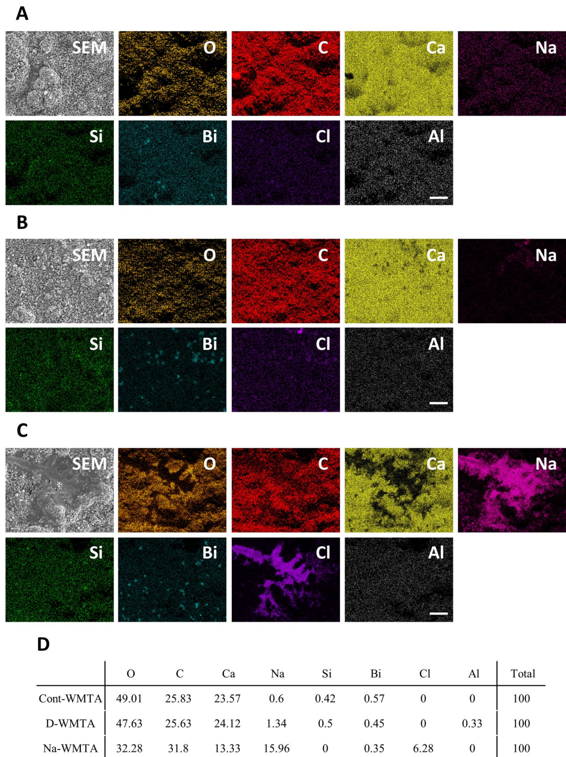
Figure 3. Elemental mapping by energy-dispersive X-ray analysis of WMTA discs immersed in NaOCl. EDX elemental mapping micrographs of Cont-WMTA ( A ), D-WMTA ( B ), and Na-WMTA ( C ). SEM, SEM micrographs; O (orange); C (red); Ca (yellow); Na (pink); Si, (green); Bi, (blue); Cl, (purple); Al, (white). Original magnification: \times 1000 . Bars = 20 \mu\text{m} . ( D ) Atomic percentage (At%) of Cont-WMTA, D-WMTA, and Na-WMTA.
