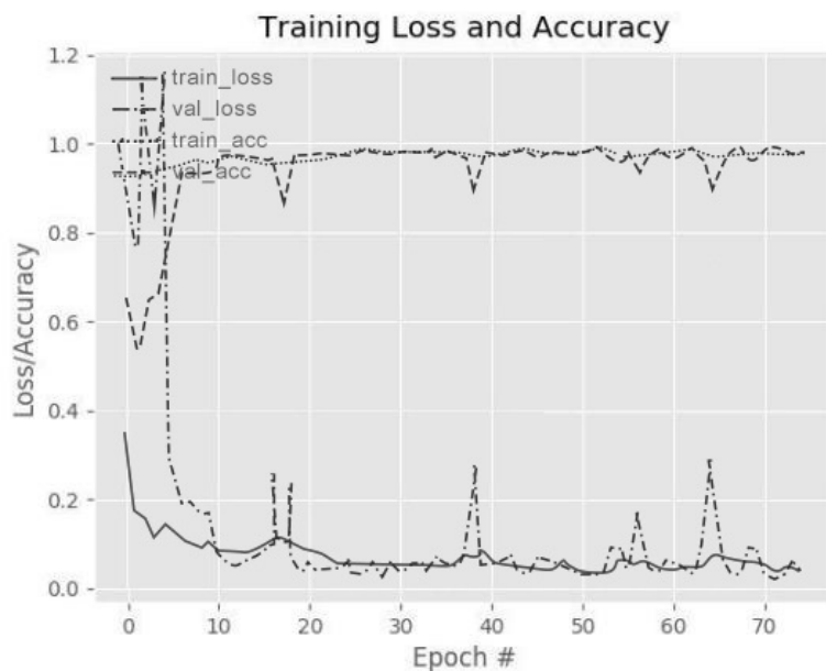
FIGURE 6. Loss & accuracy
