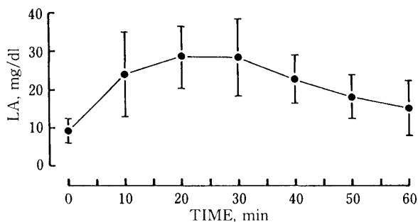
Fig. 3 The mean values of venous blood lactate concentrations during prolonged exercise.
