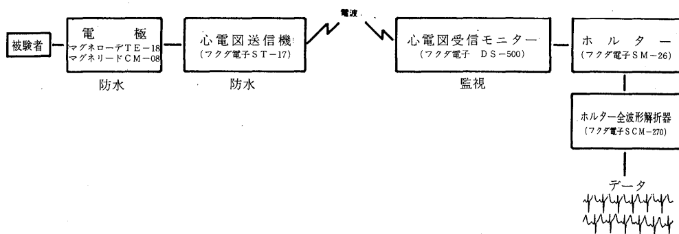
Fig.1. System for ECG recorder in swimming.
