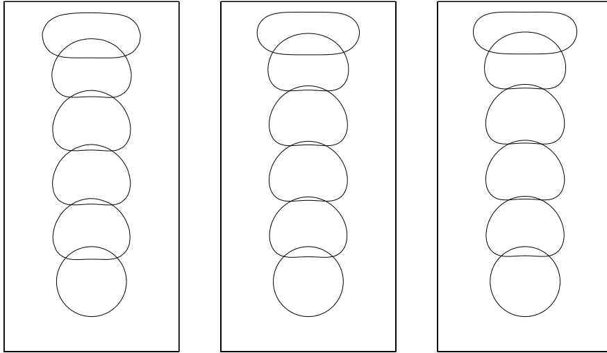
Figure 3: Interfaces at t = 0, 2, \dots, 10 solved on \mathcal{T}_{1/16} (left), \mathcal{T}_{1/32} (center), and \mathcal{T}_{1/64} (right). \sigma_0 = 1 .
