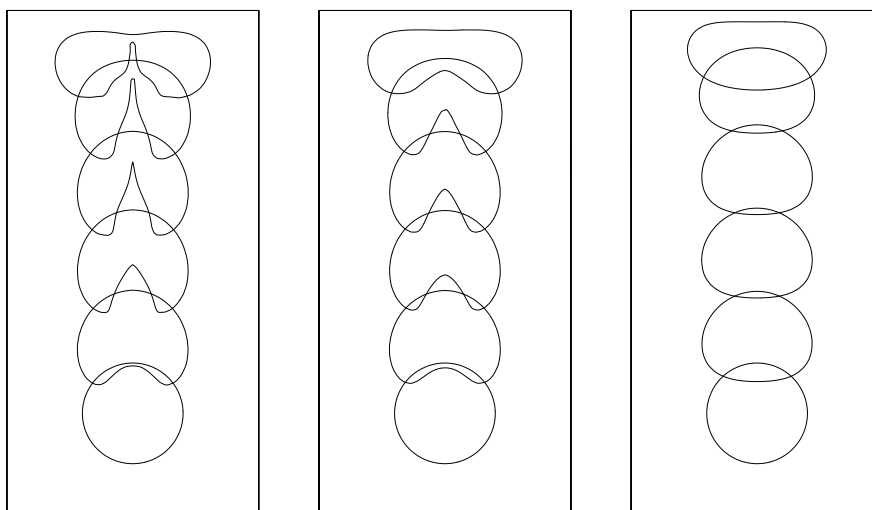
Figure 4: Interfaces at t = 0, 2, \dots, 10 , \sigma_0 = 0 (left), \sigma_0 = 0.1 (center), and \sigma_0 = 2 (right). \sigma_0 = 1 .
