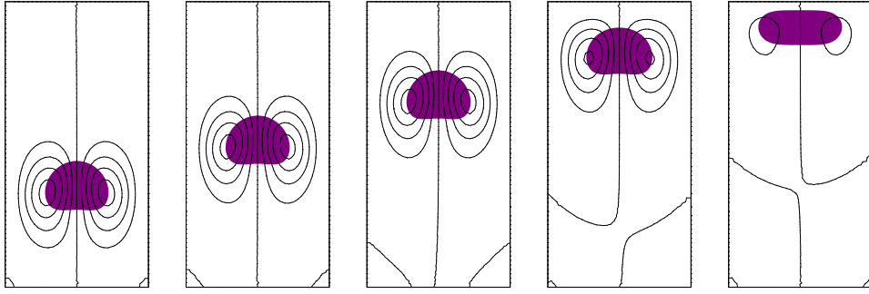
Figure 6: Interfaces and streamlines at t = 2, 4, \dots, 10 subject to the non-slip boundary conditions.
