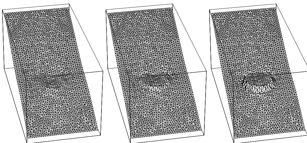
Figure 5: Elevations of the pressure at t = 5.0 . \sigma_0 = 0.0 (left), 1.0 (center), 2.0 (right).
