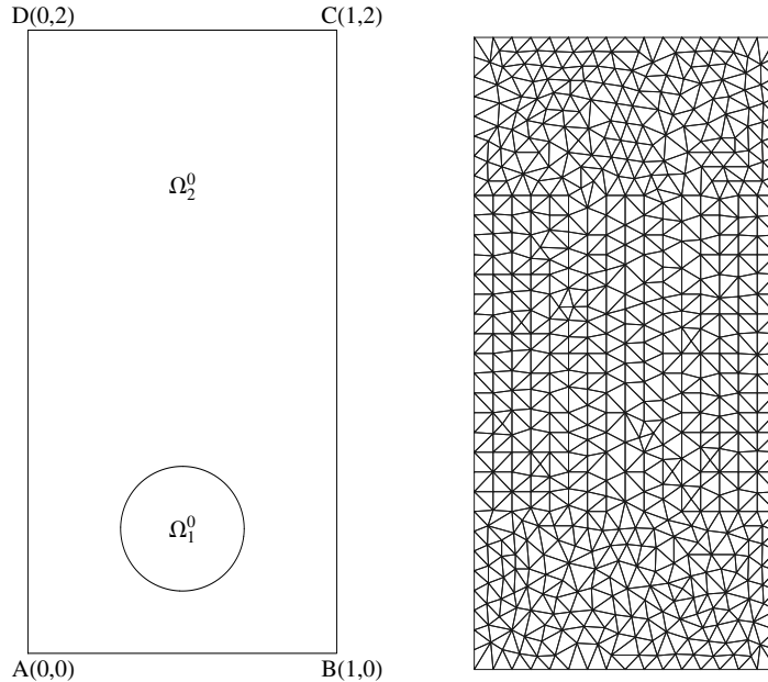
Figure 1: Statement of the problem and a mesh \mathcal{T}_{1/16} .
