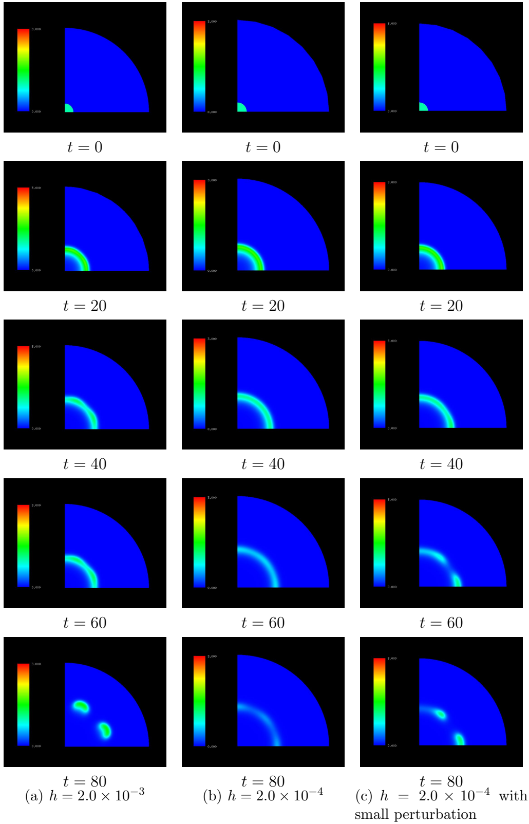
Fig. 15. Unstable expanding ring pattern in the Gray-Scott model
