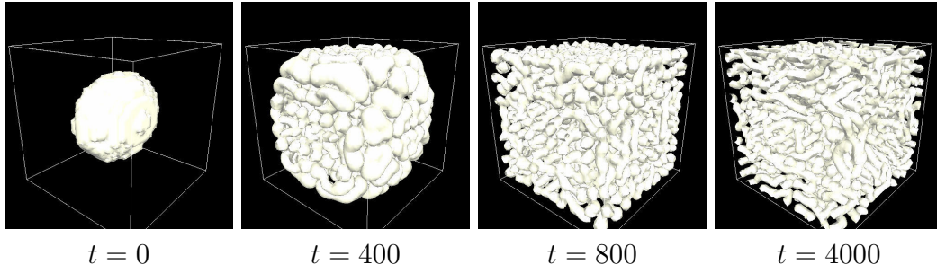
Fig. 8. Snap shots of the isosurface ( v = 0.2 ) of the numerical results of the three dimensional Gray-Scott model ( d_u = 2.5 \times 10^{-5} , d_v = 5.0 \times 10^{-6} , A = 0.02 , \alpha = 0.077 ).
