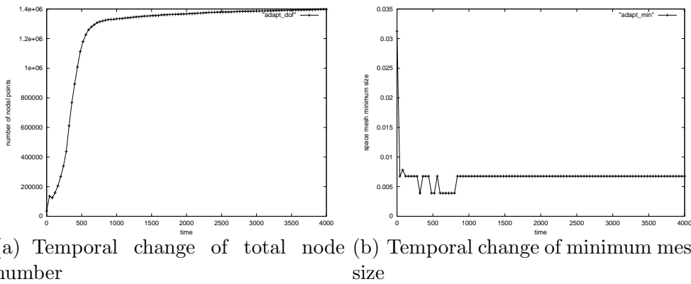
Fig. 9. Total mesh number and minimum mesh size in Fig.8.
