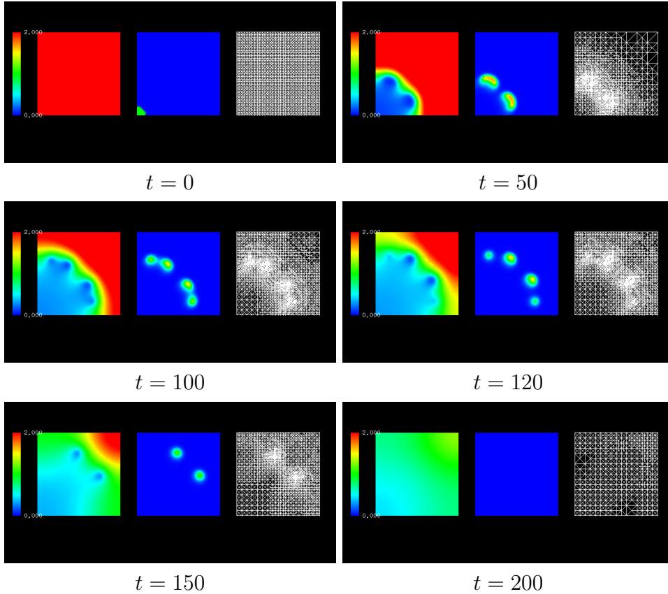
Fig. 2. Snap shots of u , v and mesh from the numerical results of the Gray-Scott model ( d_u = 11.5 \times 10^{-4} , d_v = 1.0 \times 10^{-4} , A = 0 , \alpha = 0.25 )
