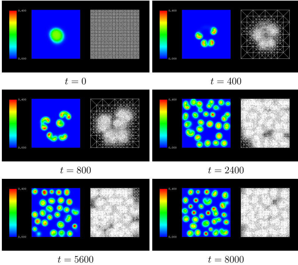
Fig. 3. Snap shots of v and mesh from the numerical results of the Gray-Scott model ( d_u = 2.0 \times 10^{-5} , d_v = 10^{-5} , A = 0.02 , \alpha = 0.077 )
