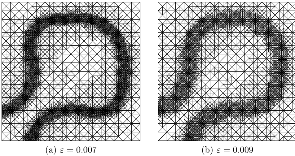
Fig. 13. Typical mesh profile of eq.(1.1) at t = 4
