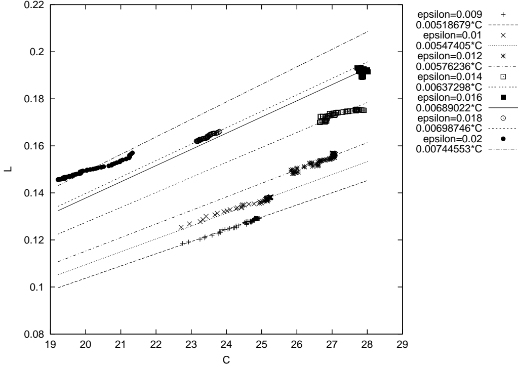
Fig. 10. Compression rate v.s. localization index on the activator-inhibitor system
