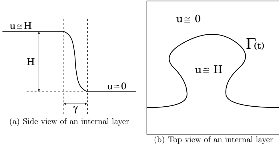
Fig. 12. Profile of a typical internal layer
