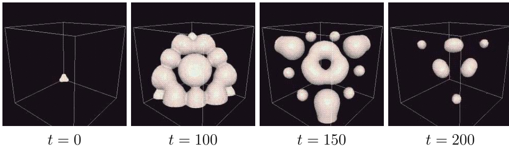
Fig. 4. Snap shots of the isosurface ( v = 0.1 ) of the numerical results of the three dimensional Gray-Scott model without supply ( d_u = 11.5 \times 10^{-4} , d_v = 1.0 \times 10^{-4} , A = 0 , \alpha = 0.25 ).
