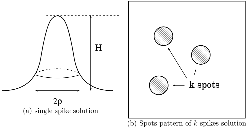
Fig. 14. Profile of a typical spike solution
