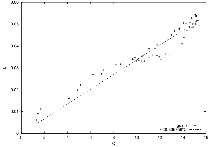
(a) The Gray-Scott model without supply ( A = 0 )
