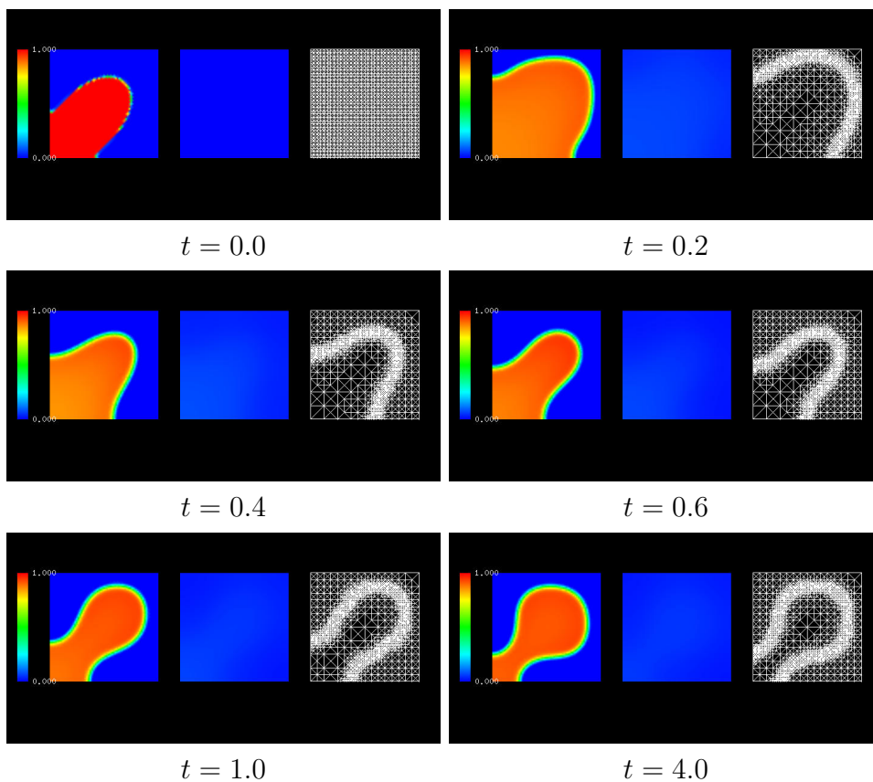
Fig. 1. Snap shots of u , v and mesh from the numerical results of the activator-inhibitor system ( \varepsilon = 0.01 , \tau = 0.1 , d = 1.0 , a = 0.25 , \lambda = 10.0 )
