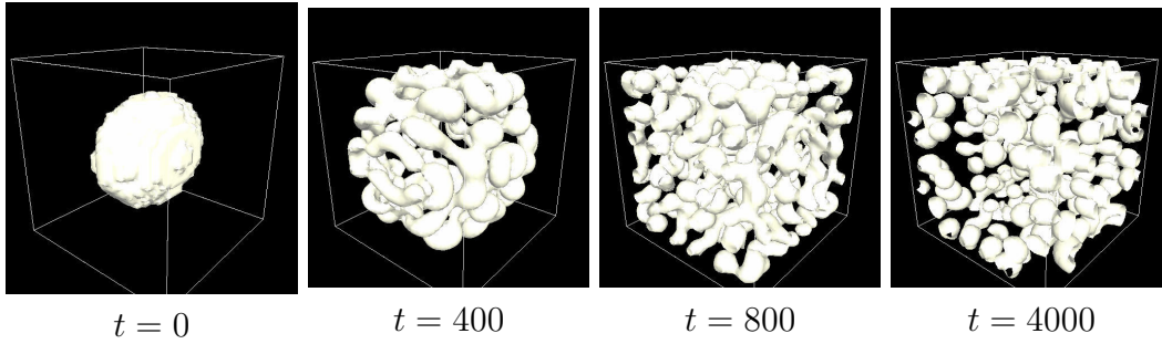
Fig. 6. Snap shots of the isosurface ( v = 0.2 ) of the numerical results of the three dimensional Gray-Scott model ( d_u = 2.0 \times 10^{-5} , d_v = 10^{-5} , A = 0.02 , \alpha = 0.077 ).
