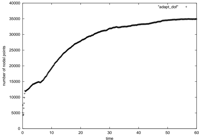
Fig. 16. Temporal change of number of nodal points in Fig.15(b).
