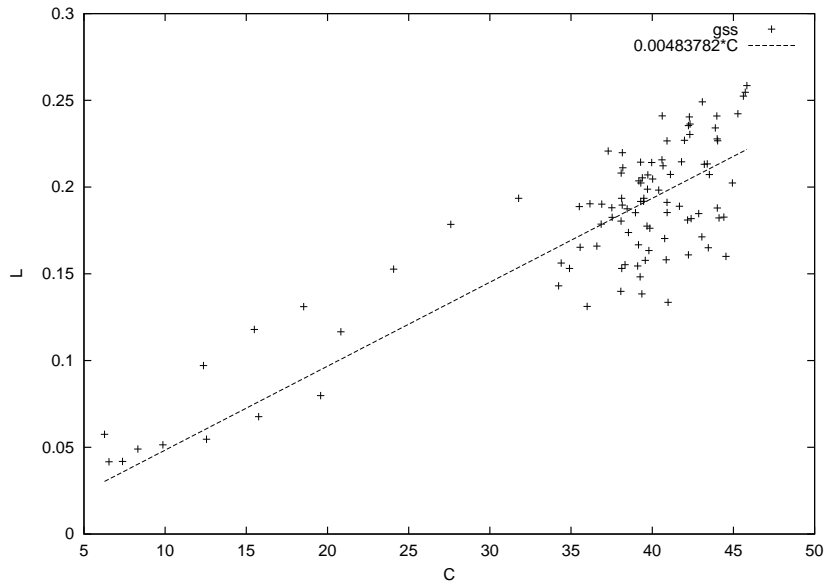
(b) The Gray-Scott model with supply ( A = 0.02 )
