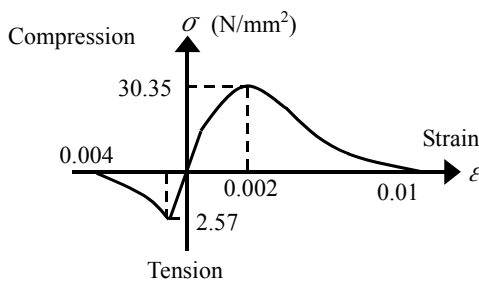
(a) Material model of concrete
