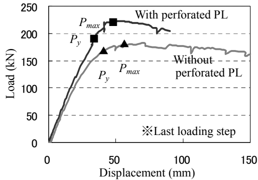
Fig.10 Load-displacement curve.
