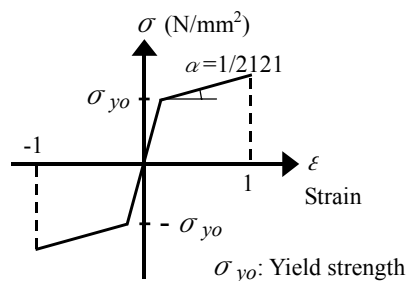
(b) Material model of steel
