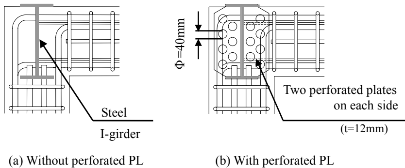
Fig.8 Detail of knee joint.
