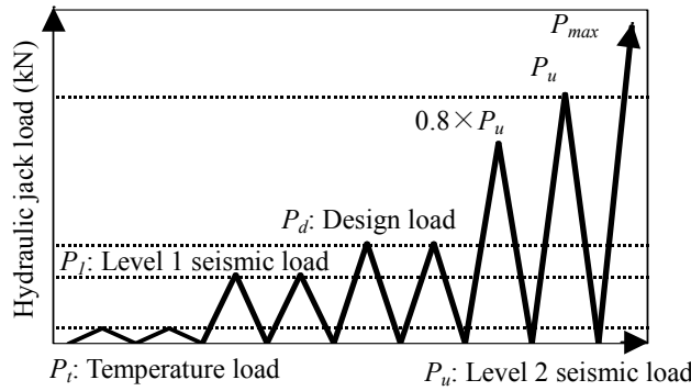
Fig.9 Loading step.
