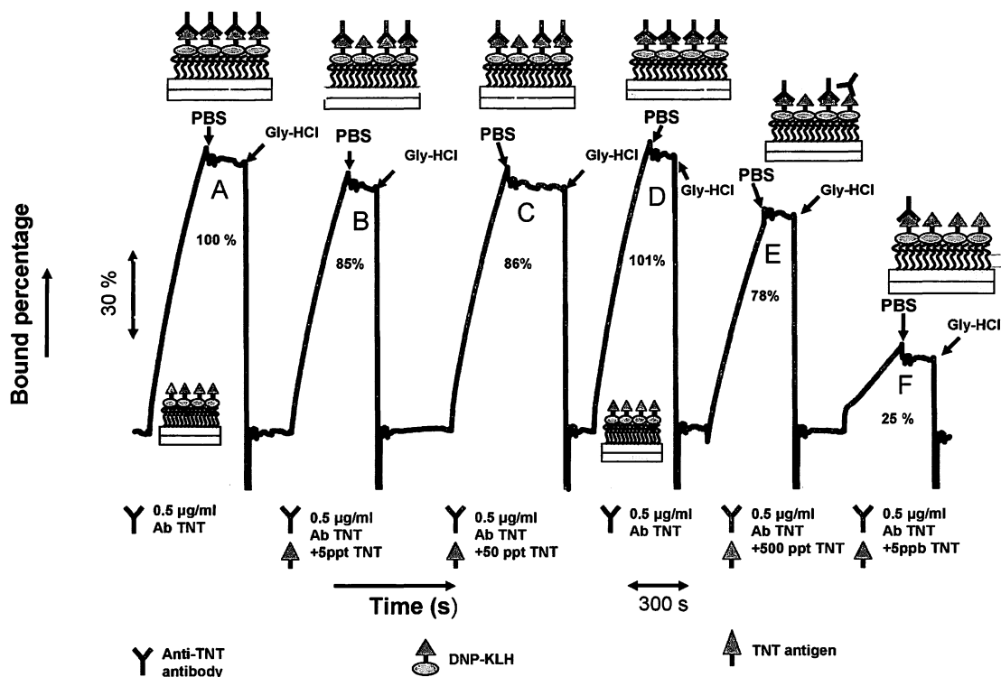
Fig. 3. SPR sensorgram of competitive inhibition assay performed using 0.5 \mu\text{g/ml} anti-TNT antibody concentration and TNT as an analyte in varying concentrations.
