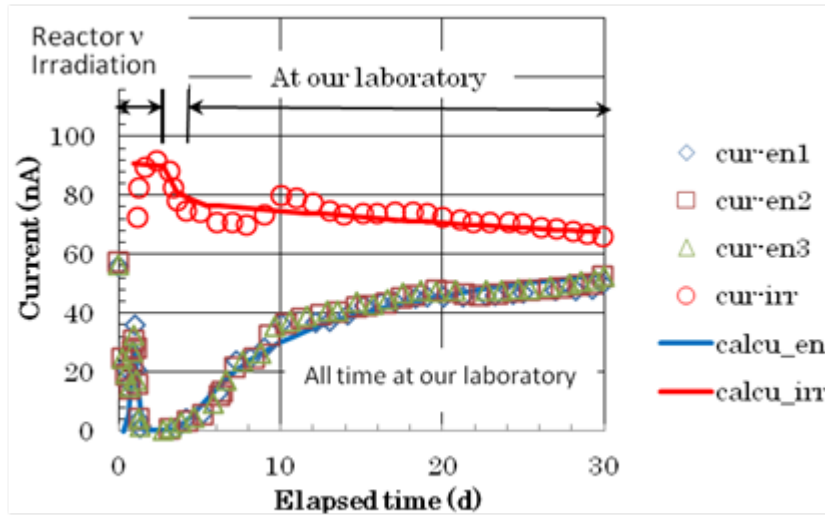
Fig. 2 Output current of the apparatus. The lower marks of three types are the results for the experiments performed under environmental conditions in a laboratory at Kyushu University, while the upper marks show the results obtained under reactor-neutrino irradiation and subsequent environmental conditions 7) . The solid curves indicate calculation results.
