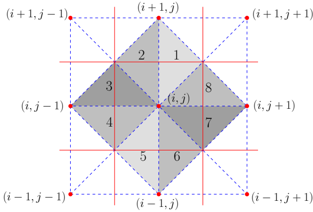
Figure 5: Co-volume p associated with a couple (i, j) and set of 8 triangles \mathcal{N}_{i,j} denoted by numbers 1 to 8.
