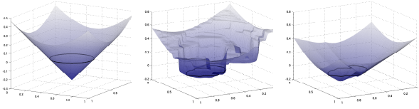
Figure 3: Example of segmentation function. Initial segmentation function u_0 (left), segmentation function u for ( t > 0 ) (middle), restored SDF (right).
