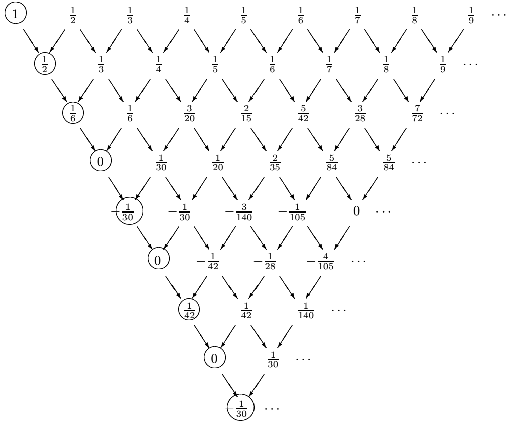
Figure 1: Akiyama-Tanigawa triangle
