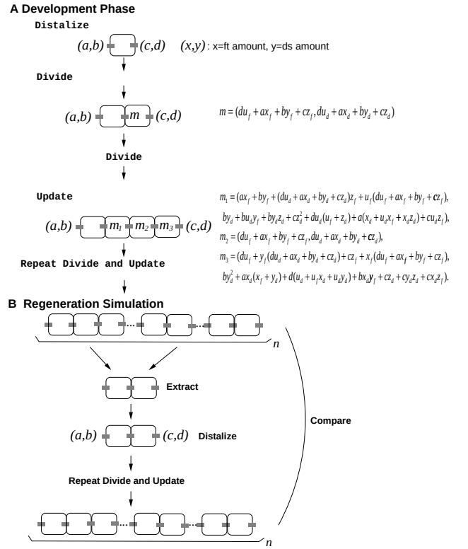
Figure 2: The development phase and the regeneration simulation. A: The Development phase. Distalize procedure makes each cell distalized ( (l_{ft}, l_{ds}, r_{ft}, r_{ds}) is set (a, b, c, d) in the figure). Divide procedure makes each cell divide (a newly cell wall is created with heterodimers m = (ft, ds) = (du_f + ax_f + by_f + cz_f, du_d + ax_d + by_d + cz_d) in the figure). Update procedure updates inner heterodimers ( m_1, m_2 , and m_3 in the figure). B: The regeneration simulation. When the cell number turns n , part of the cell chain is extracted and developed again. The cell chain thus obtained is compared with the original one (See the text.)
