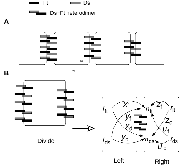
Figure 1: A schematic illustration of the Ds-Ft system. A: The heterodimeric bridges are formed by Ds and Ft molecules between cells. The gradient of Ds-Ft heterodimers across the cells is considered to provide cells with a polarity or regeneration cue [20]. B: During the cell division, surplus Ft, Ds and their heterodimers are deemed redistributed on the cell surface. l_{ft,ds} designates the amounts of Ft and Ds, respectively, of heterodimers on the left-side surface of the left cell. Likewise, r_{ft,ds} designates those on the right-side surface of the right cell, and n_{ft,ds} designates those on the left-side surface of the right cell. \{x, y, z, u\}_{f,d} denote the redistribution ratio of heterodimers (see the text for details).
