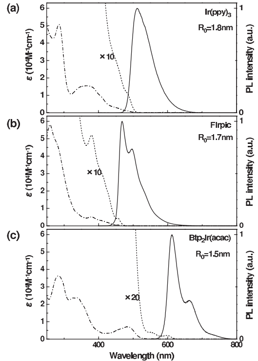
FIG. 3. Absorption (broken line) and PL spectra (solid line) of (a) Ir(ppy) _3 , (b) Flrpic, and (c) Btp _2 Ir(acac) in methylenechloride ( 2 \times 10^{-5} M). The dotted lines show the absorption value expanded 10 times for the Ir(ppy) _3 and Flrpic and 20 times for the Btp _2 Ir(acac). The Förster radii ( R_0 ) obtained by the spectral overlap in Eq. (3) are shown.
