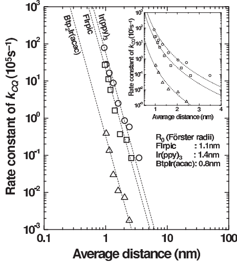
FIG. 2. Dependence of concentration-quenching rate constants ( k_{CQ} ) on average distance ( R ) plotted by double logarithmic axis for three complexes. The Föster radii ( R_0 ) obtained by fitting the k_{CQ} - R relations are shown. Inset also shows R vs k_{CQ} by linear ( R )-logarithmic ( k_{CQ} ) axes.
