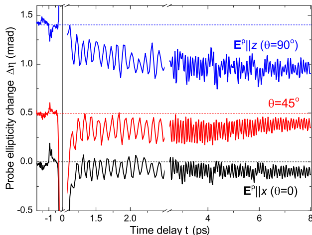
FIG. 2: (Color online) Probe ellipticity change \Delta\eta as a function of the pump-probe time delay, t , measured at three different polarizations, \theta , of the pump pulses. The probe polarization is \phi = 45^\circ .
