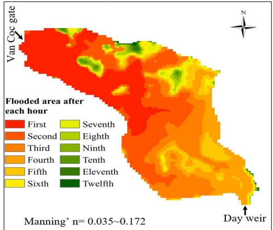
Fig. 4 Flooded areas after each hour in the case of a discharge flow of 2,500 m 3 /s at the
