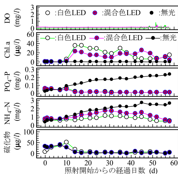
Fig. 2 Results of continuous and periodical water quality observations under the low light condition
