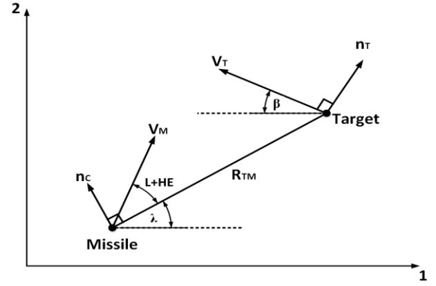
Fig. 1. Two-dimensional missile-target engagement geometry.
