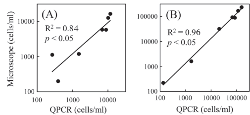
Fig. 4. Relation analysis between cell densities calculated by microscope and quantitative PCR (QPCR) in C. marina (A) and H. akashiwo (B) by Pearson's correlation coefficient test.
