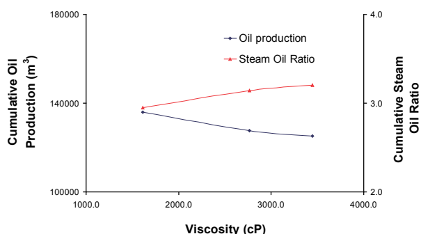
Fig. 4 Effect of viscosity on cumulated oil production and steam oil ratio.
