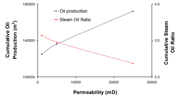
Fig. 3 Effect of permeability on cumulated oil production and steam oil ratio.
