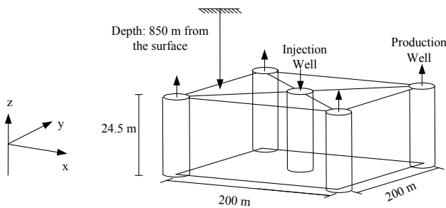
Fig. 2 Schematic diagram of 5-spot pattern and oil well.
