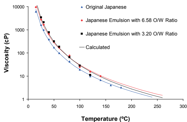
Fig. 1 Effect of temperature on viscosities of Japanese oil and its emulsions.
