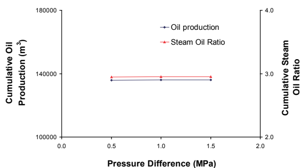
Fig. 5 Effect of pressure difference on cumulated oil production and steam oil ratio.
