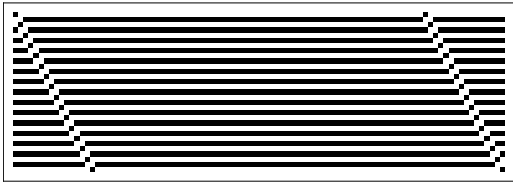
Fig. 3: An example of configurations of CA(3, 3)
