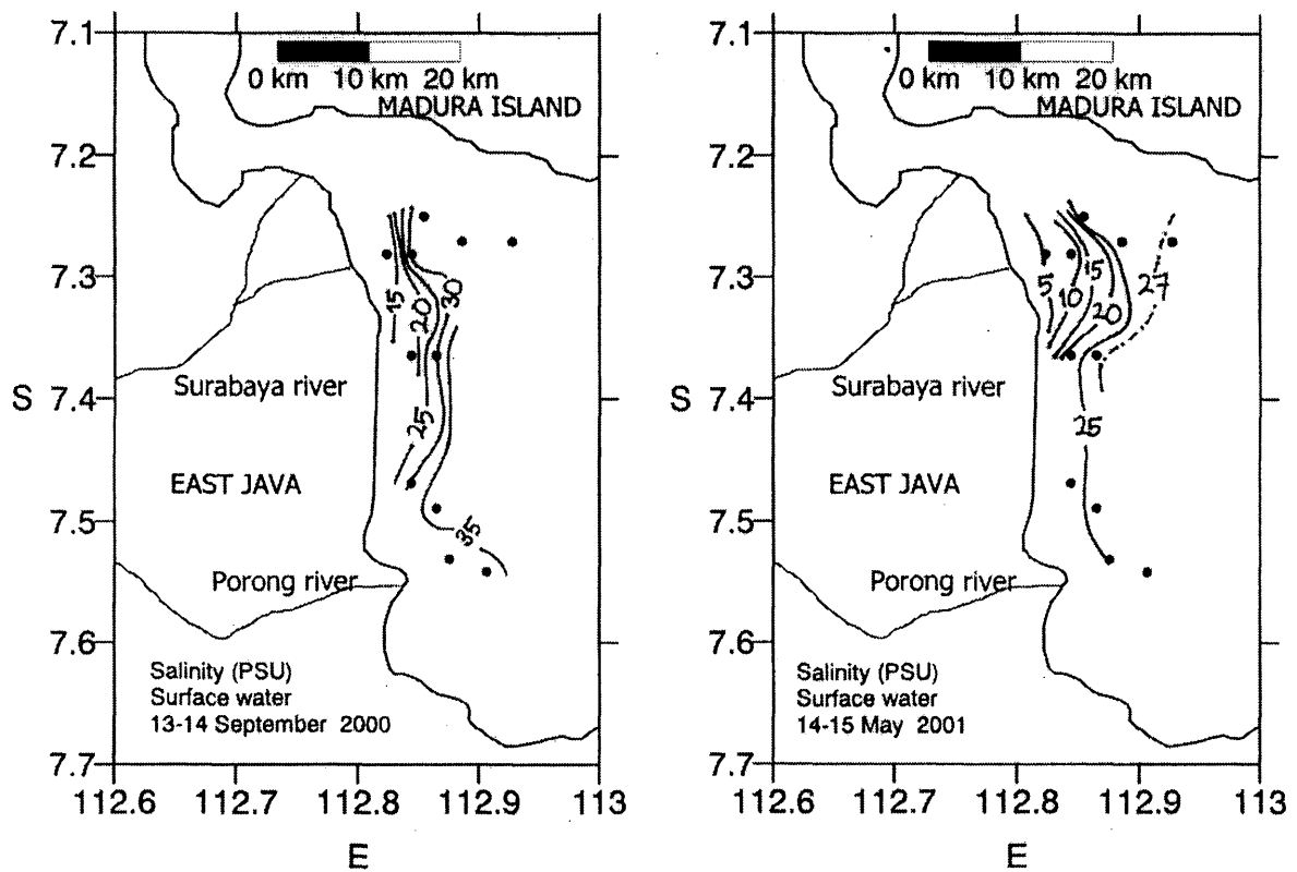
Fig. 5 Salinity of surface water
