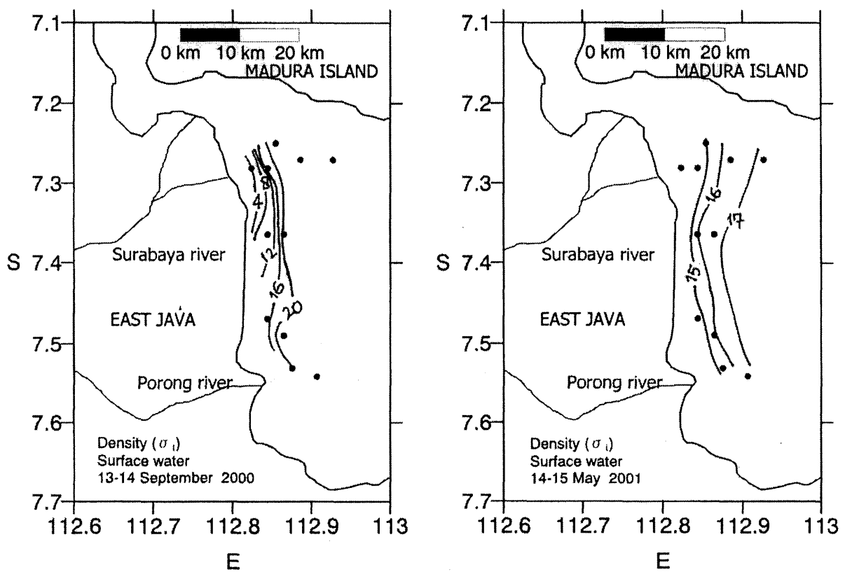
Fig. 6 Density ( \sigma_t ) of surface water
