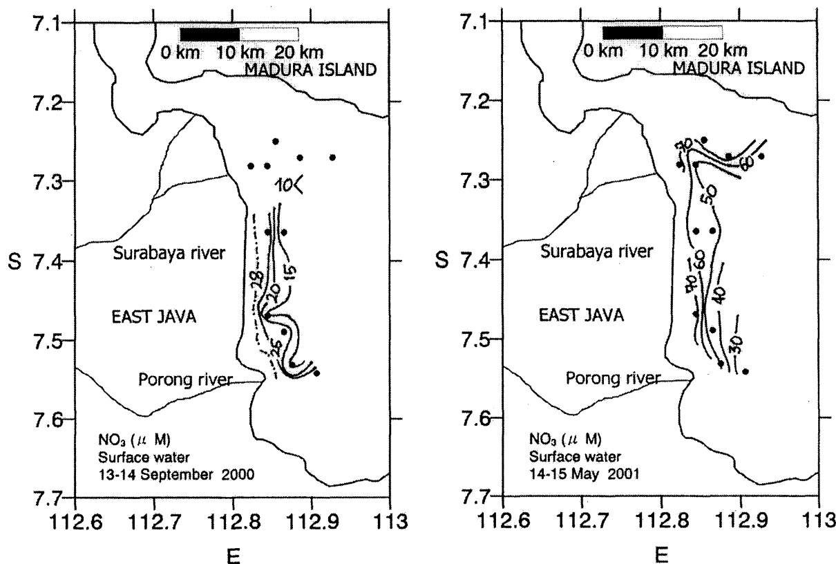
Fig. 9 Nitrate ( \mu M) of surface water
