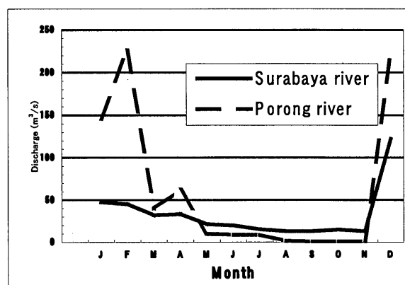
Fig. 3 Discharge of Surabaya river and Porong river in 1997.
