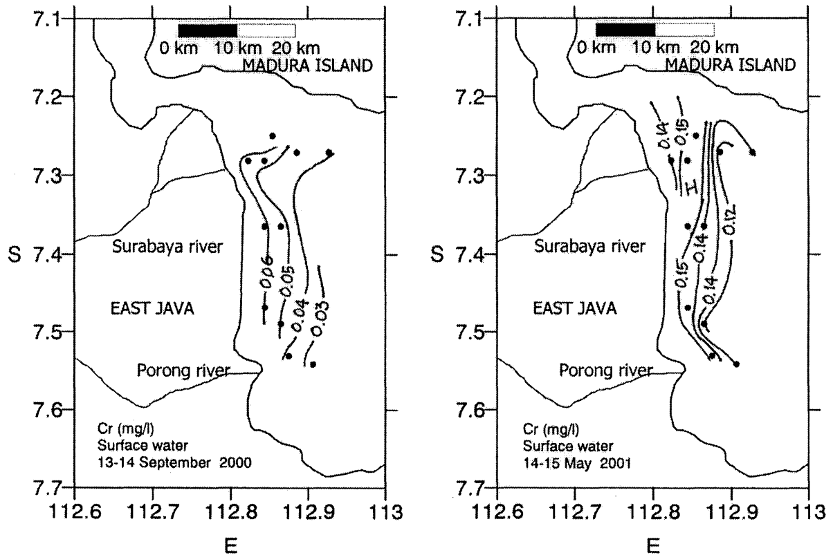
Fig. 8 Chromium (mg/l) of surface water
