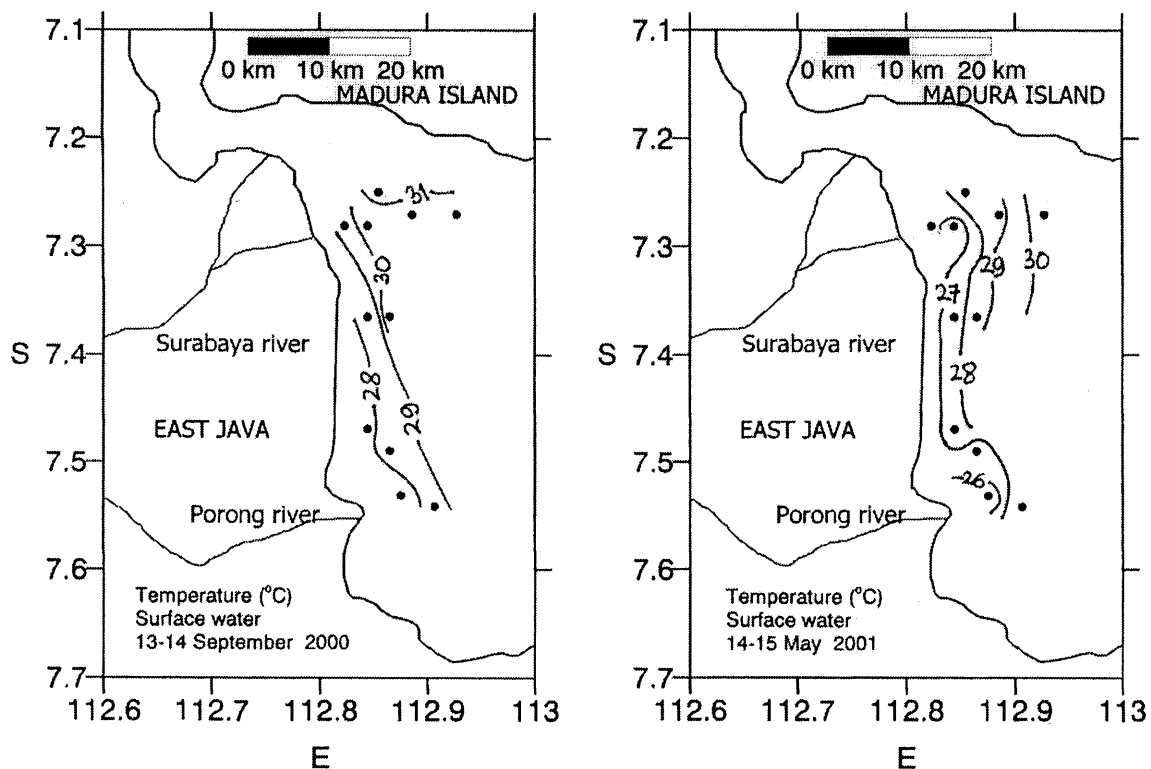
Fig. 4 Temperature of surface water
