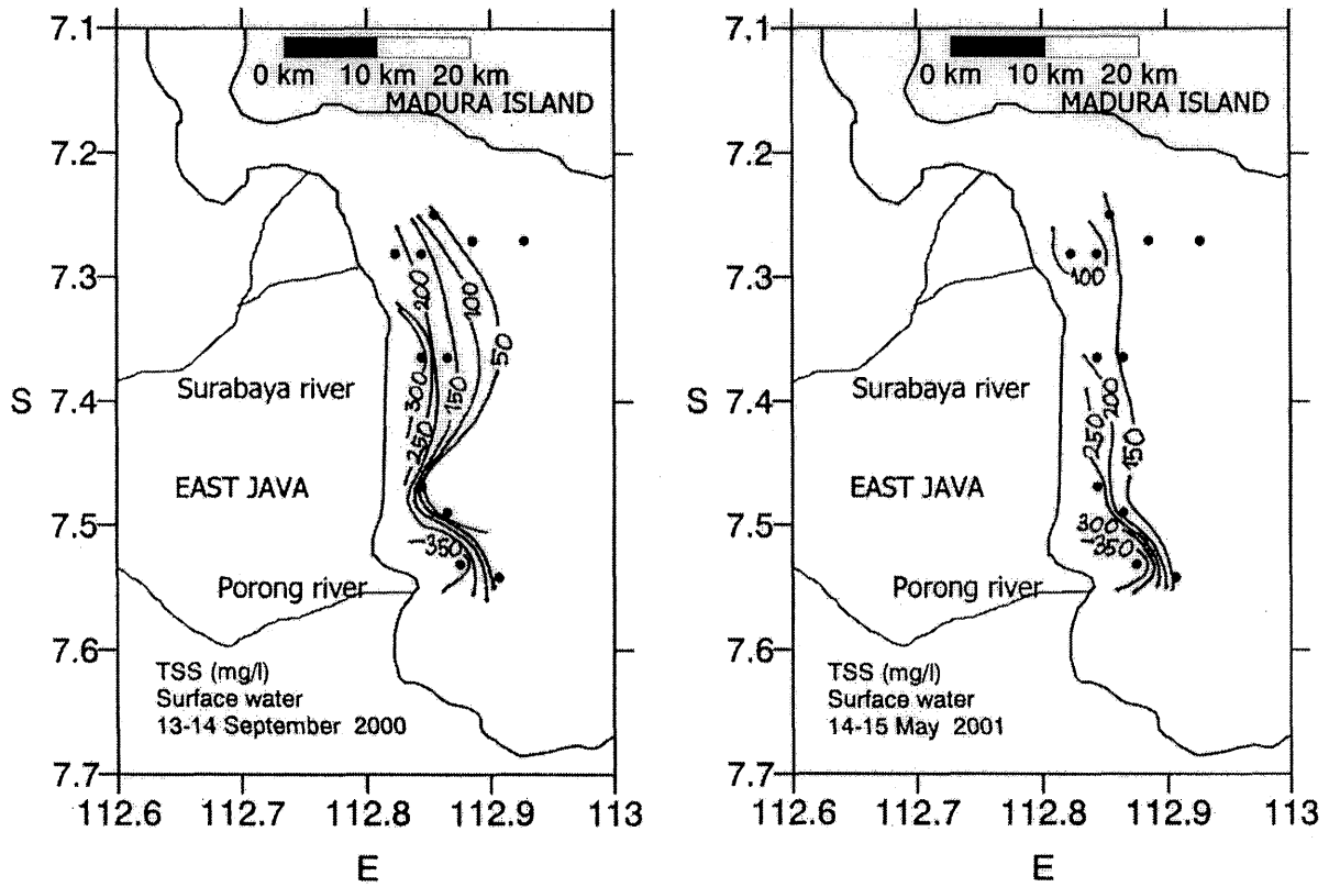
Fig. 7 Total suspended solid (mg/l) of surface water
