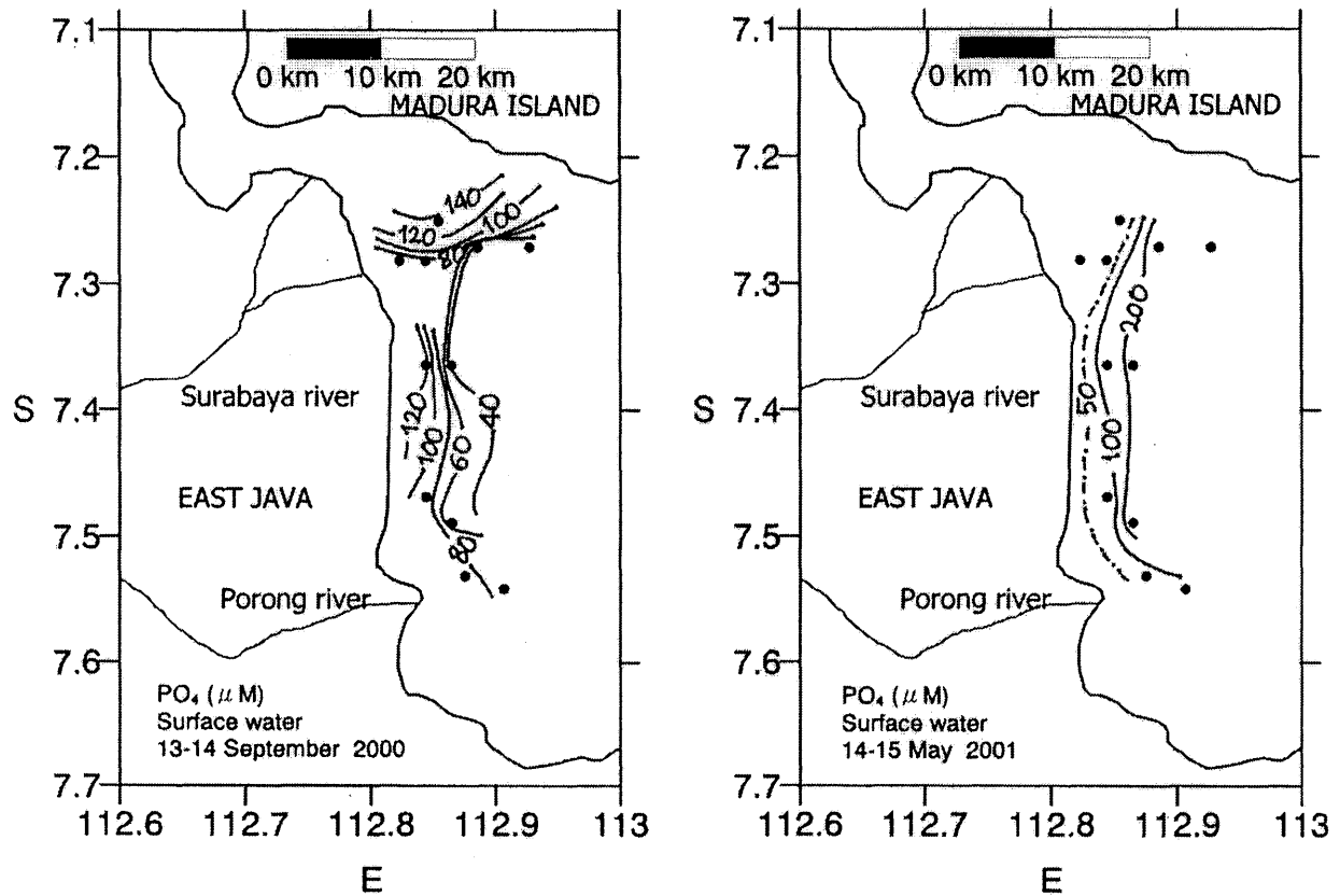
Fig. 11 Phosphate ( \mu\text{M} ) of surface water
