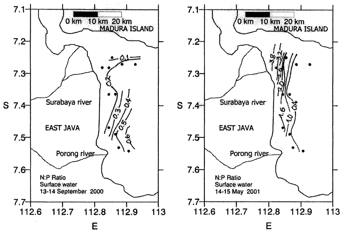
Fig. 12 N:P ratio
