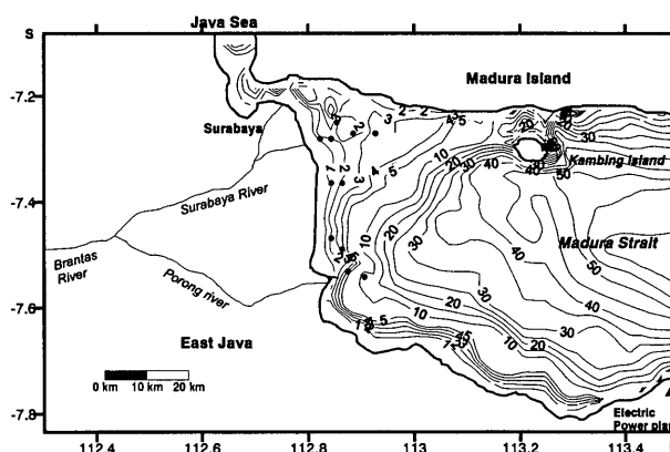
Fig. 2 Study area and bottom topography. Numbers show depth in meter.
