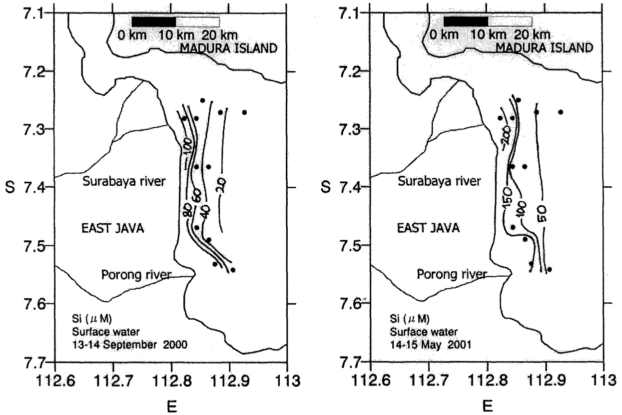
Fig. 10 Silicate ( \mu\text{M} ) of surface water
