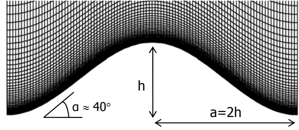
Fig.3 Structured computational mesh used in the vicinity of the isolated-hill in the RIAM-COMPACT® simulation.
