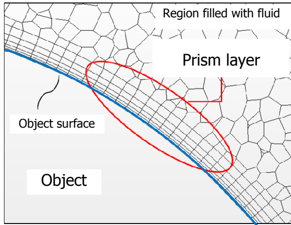
Fig.1 Polyhedral mesh and prism layer mesh
