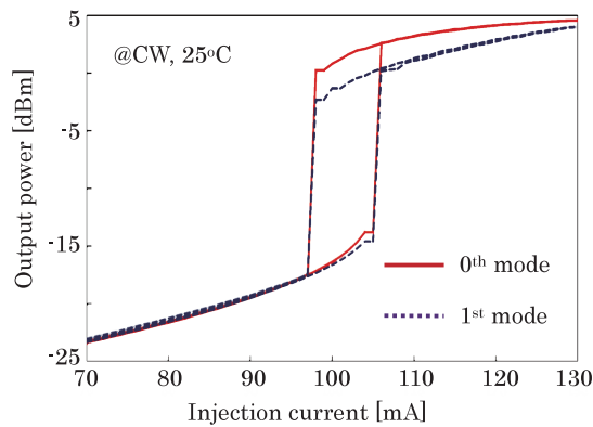
Fig. 8 P-I characteristics of the fabricated novel active-MMI BLDs(@CW, 25°C).
