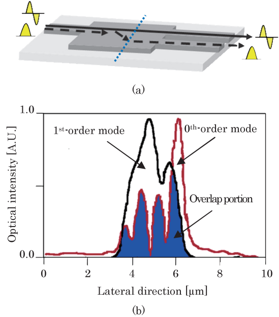
Fig. 5 Optical field profiles in the novel active-MMI waveguide area. (a) Propagation paths of 0 th -order and 1 st -order modes light, (b) optical field profiles corresponding to the position indicated in (a) (blue dotted line). The blue colour indicates overlap portion of the optical field profiles in the MMI region.
