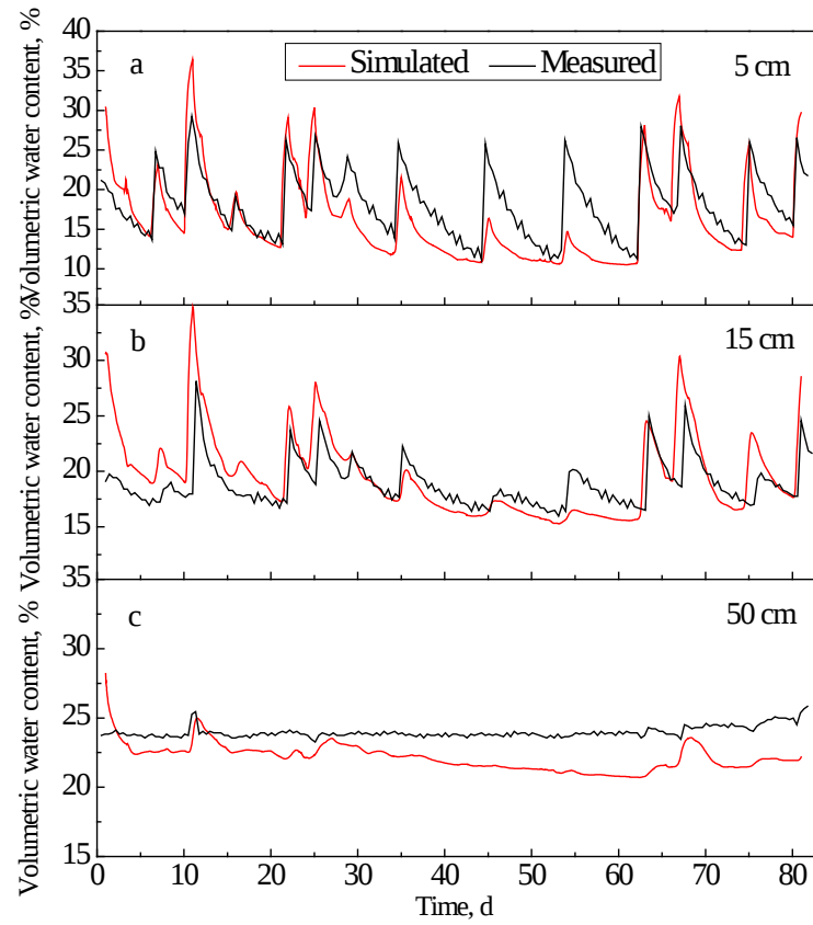
Fig. 9 Comparison between simulated and measured water content at three different depths, (a) 5 cm, (b) 15 cm, and (c) 50 cm.
