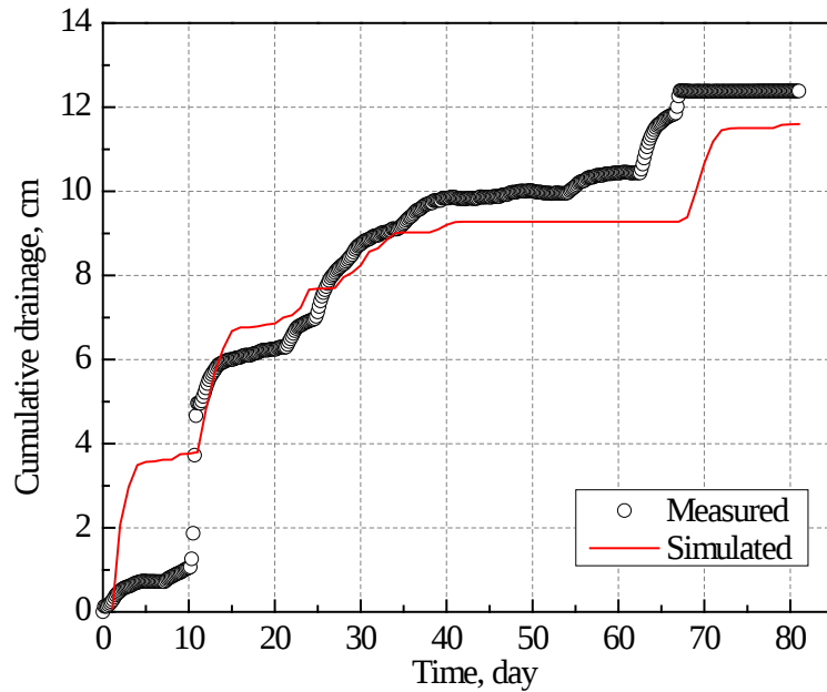
Fig. 11 Variation of cumulative drainage: comparison between simulation and measurement.
