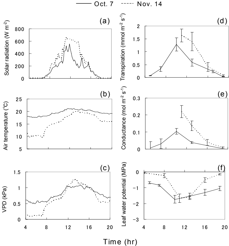
Fig. 3. Diurnal course of (a) solar radiation, (b) air temperature, (c) vapor pressure deficit (VPD), (d) leaf transpiration rates, (e) leaf stomatal conductance, and (f) leaf water potential on October 7 and November 14. Leaf transpiration rates and stomatal conductance were not measured in the early morning of November 14 due to heavy dew. October 7 was in the period with heat-pulse velocity reduction, while November 14 lies outside the period.
