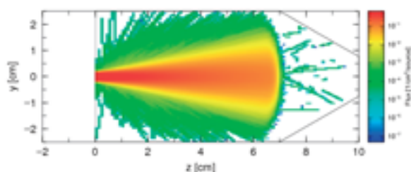
Fig.6 Two-dimensional histogram of calculated proton flux in the CsI(Tl) scintillator. The proton beam is incident from left side to detector along z axis with 4mm diameter.
