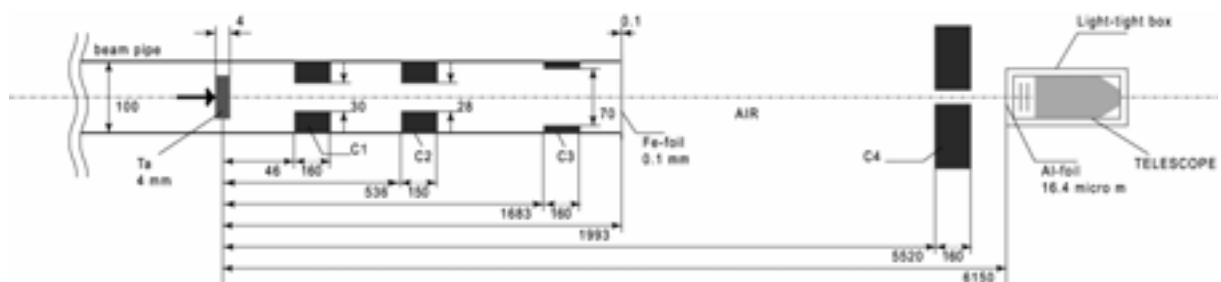
Fig.1 Experimental setup of TSL B-line. Proton beam comes from the left side of figure. C1-C4 shows the graphit collimators, and the length or thickness is given in units of mm.
