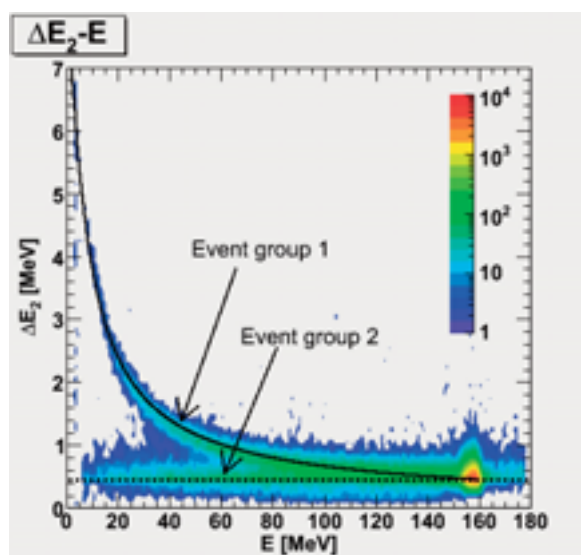
Fig.3 Tow-dimensional histogram of \Delta E_2 -E. The solid line shows the calculated energy loss in \Delta E_2 detector. Event group 1 contains the low energy tail of incident protons. Event group 2 contains the reaction losses for incident protons.
